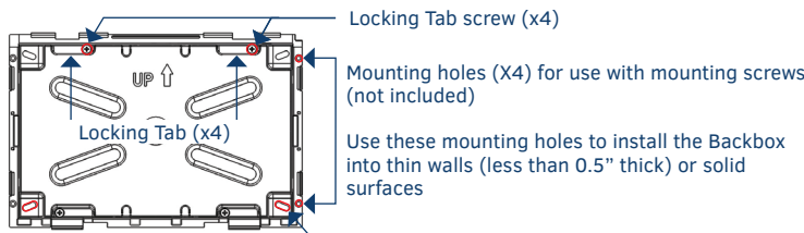
Mounting holes (x4) for installing the backbox into a Rough-In Box (screws not included)
