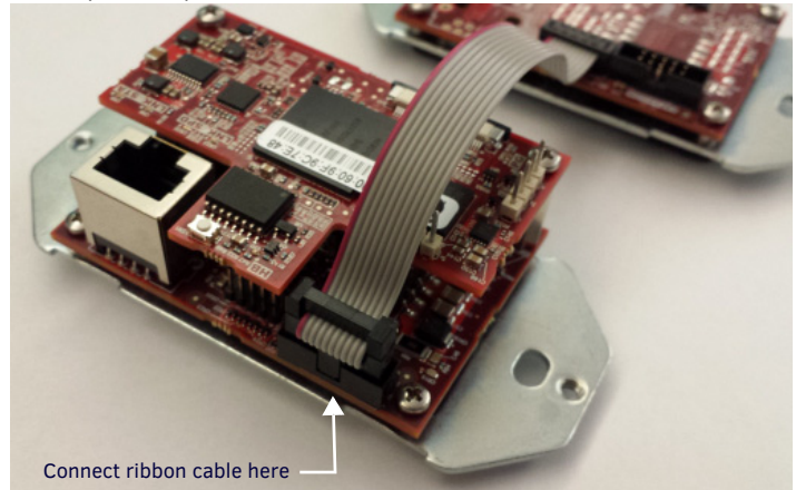
FIG. 1 DAISY-CHAIN CONNECTION BETWEEN THE MET-7E AND AN ETHERNET EXPANSION KEYPAD NOTE: If you are installing a single expansion keypad into a 3-gang back box, install the expansion keypad in the space immediately adjacent to the primary Ethernet keypad (see FIG. 2). Daisy-chaining is supported across a distance of 4" (101.6 mm).
