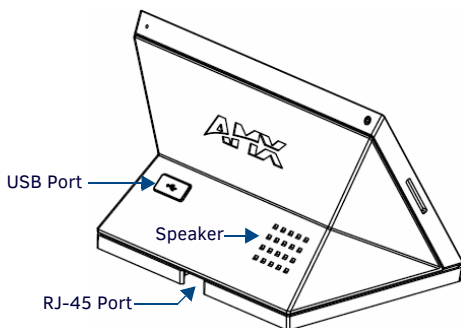
FIG. 2 MST-431 USB PORT LOCATION
