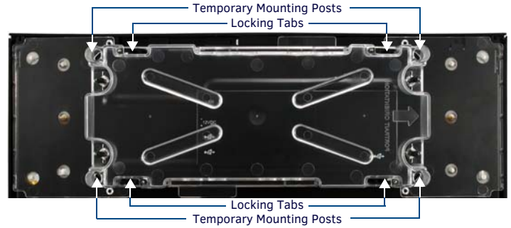
FIG. 2 MXD-1900L-PAN BACKBOX
