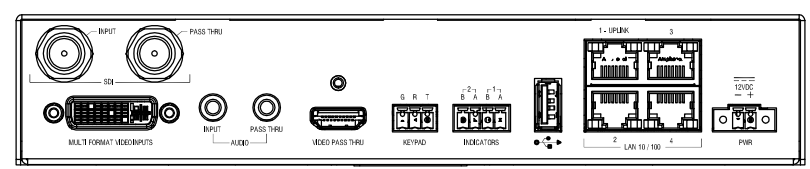
REAR VIEW
