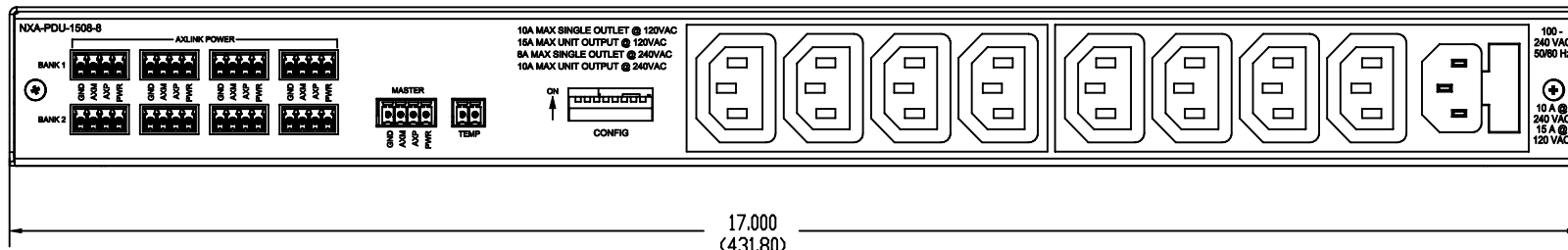
REAR VIEW
