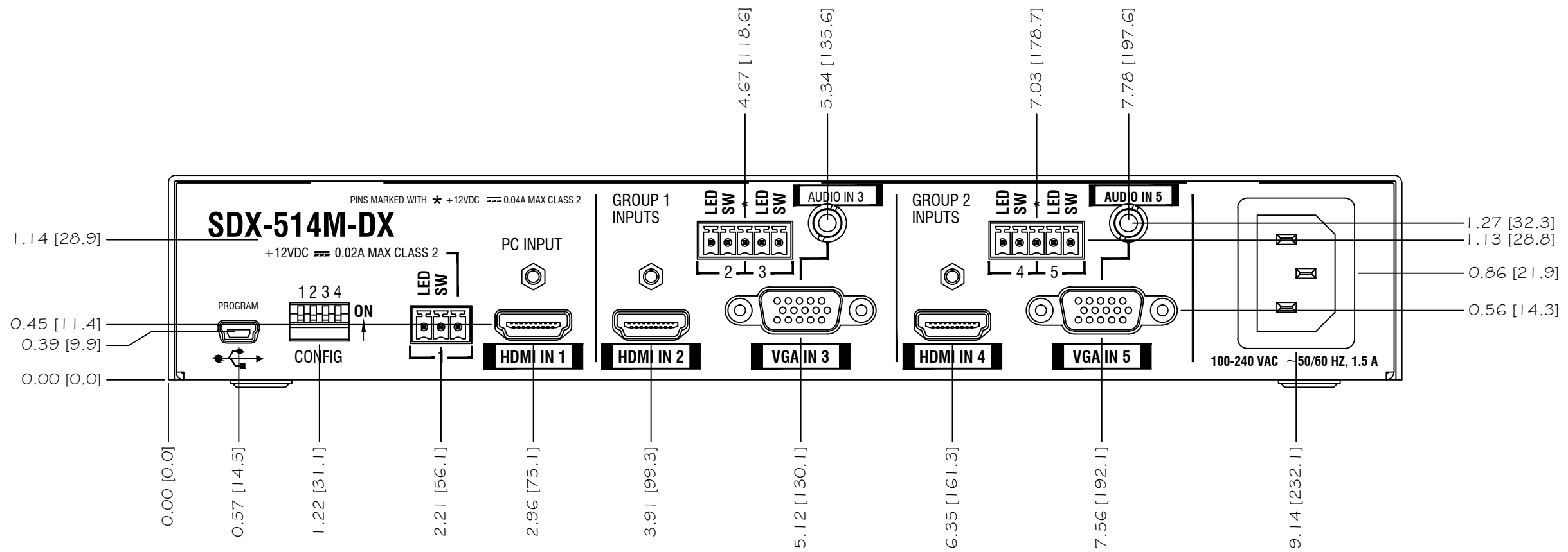
BACK VIEW
