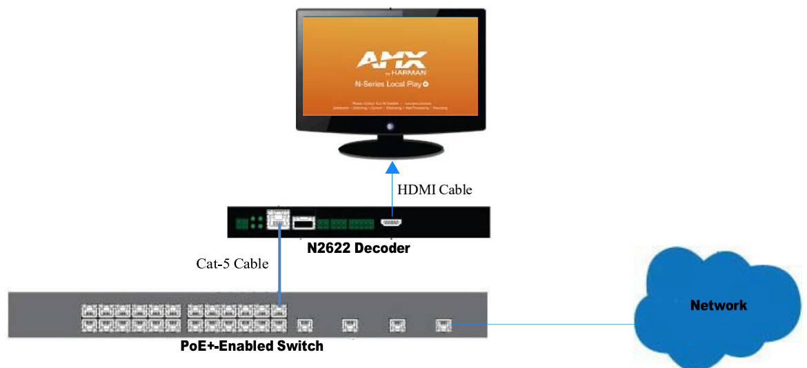
FIG. 9 Decoder Connections
