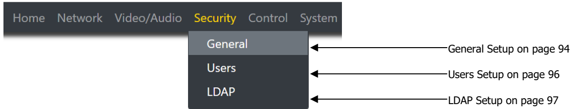
FIG. 83 Security Page
