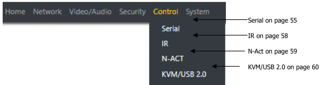
FIG. 45 Control Page
