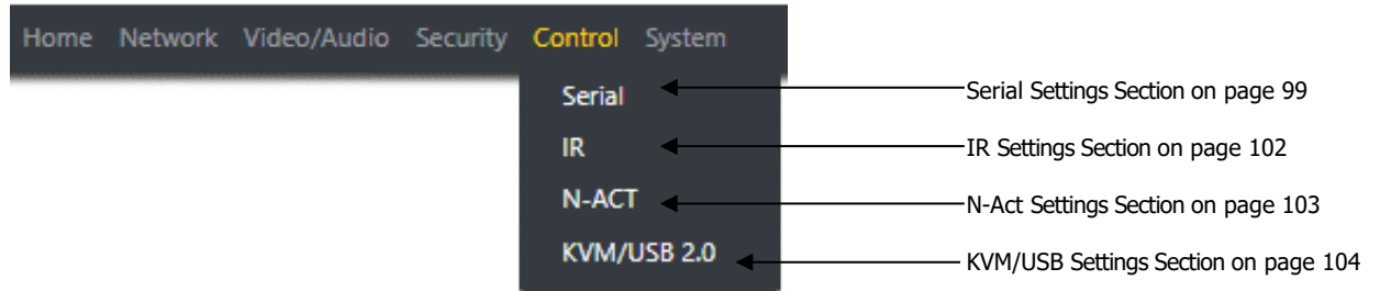
FIG. 88 Control Page
