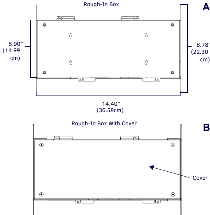
FIG. 1 CP-MXP19/20 ROUGH-IN BOX - WITH FRONT COVER
