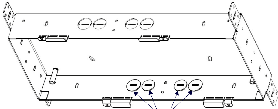
CBMXP19/20 Rough-In Box Without Cover (oblique angle)
