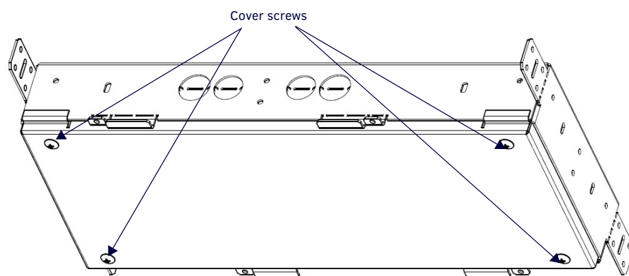
CB-MXP19/20 Rough-In Box With Cover (oblique angle)
