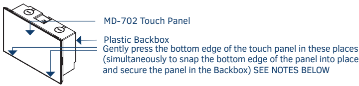
FIG. 5 SNAPPING THE BOTTOM EDGE OF THE PANEL INTO THE BACKBOX
