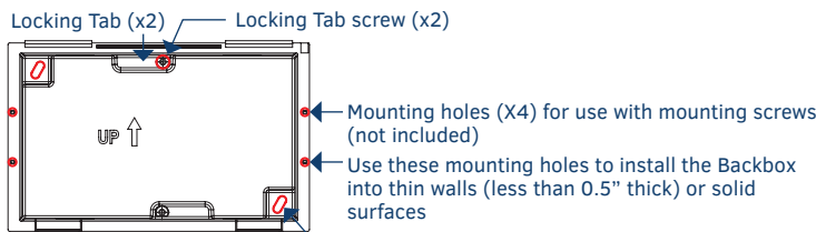
Mounting holes for installing the Backbox into a Rough-In Box (screws not included)
