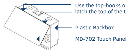
FIG. 4 ENGAGING THE TOP EDGE OF THE PANEL WITH THE TOP HOOKS ON THE BACKBOX
