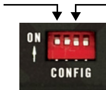
FIG. 1 CONFIGURATION DIP SWITCH
